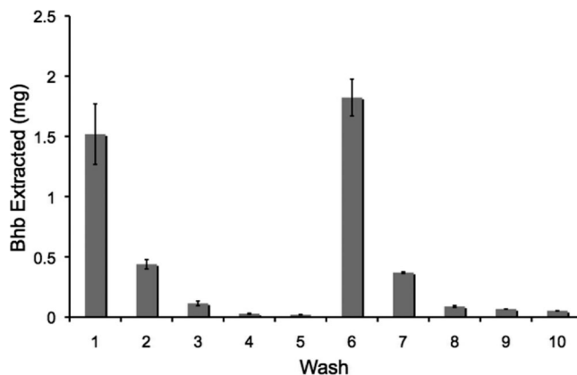
Figure 2. Bhb rebinding experiment performed on an uncharged (0% ionic groups) Bhb-imprinted polymer hydrogel. Washes 1–5 were performed using deionized water, while washes 6–10 were performed using SDS–HOAc solution.
