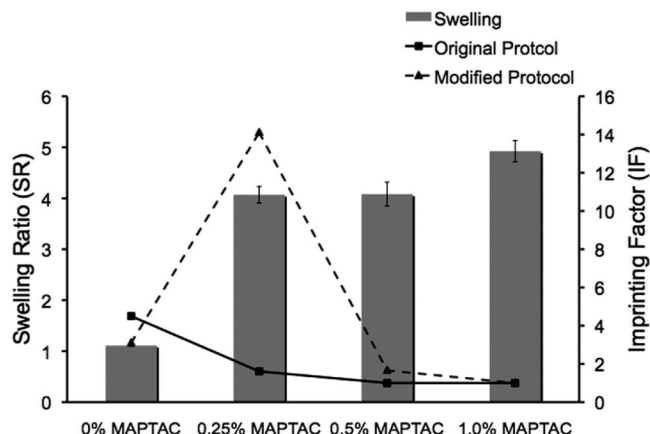
Figure 5. Swelling data and imprinting factor (IF) for gels with various amounts of positively charged MAPTAC monomer. The columns represent the swelling data, while the solid and dashed lines represent the IF of gels washed under the original and modified protocol, respectively. The peak in the dashed line at 0.25% MAPTAC represents the optimum monomer concentration for binding Bhb.
