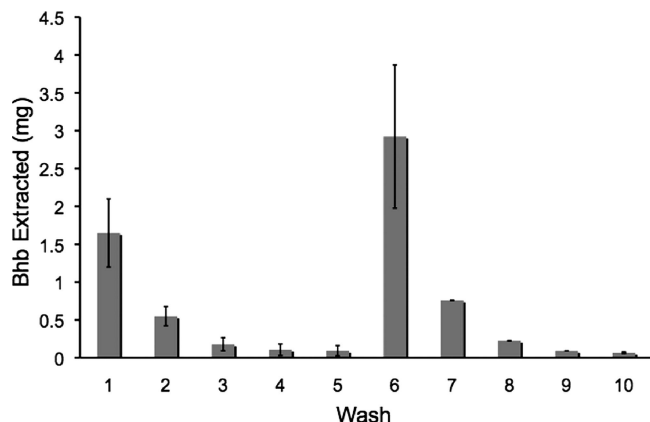
Figure 1. Wash profile for an uncharged (0% ionic groups) Bhb-imprinted hydrogel. Washes 1–5 were performed using deionized water, while washes 6–10 were performed using SDS–HOAc solution.
